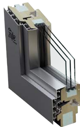
Passivhaus Aluminium Clad
